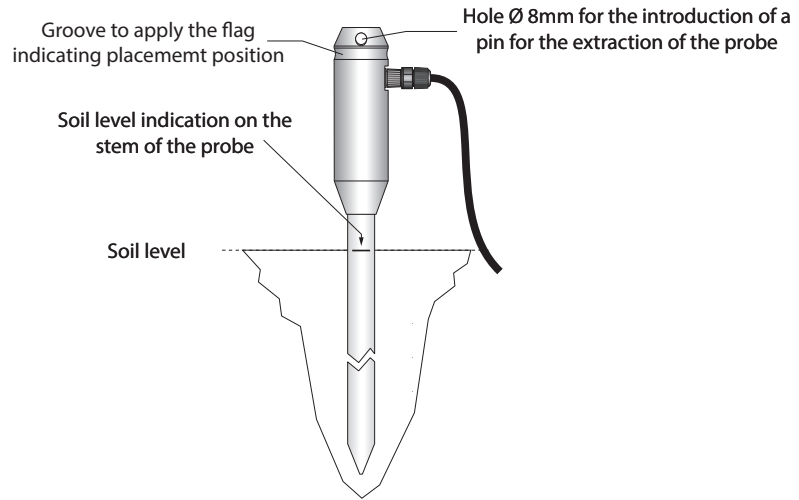
Fig. 2: installation
